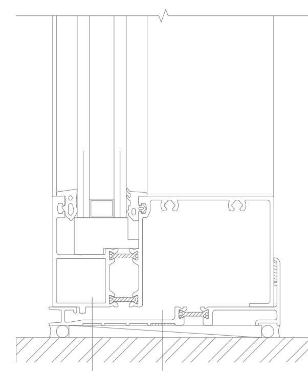
DETAIL 3 SILL
